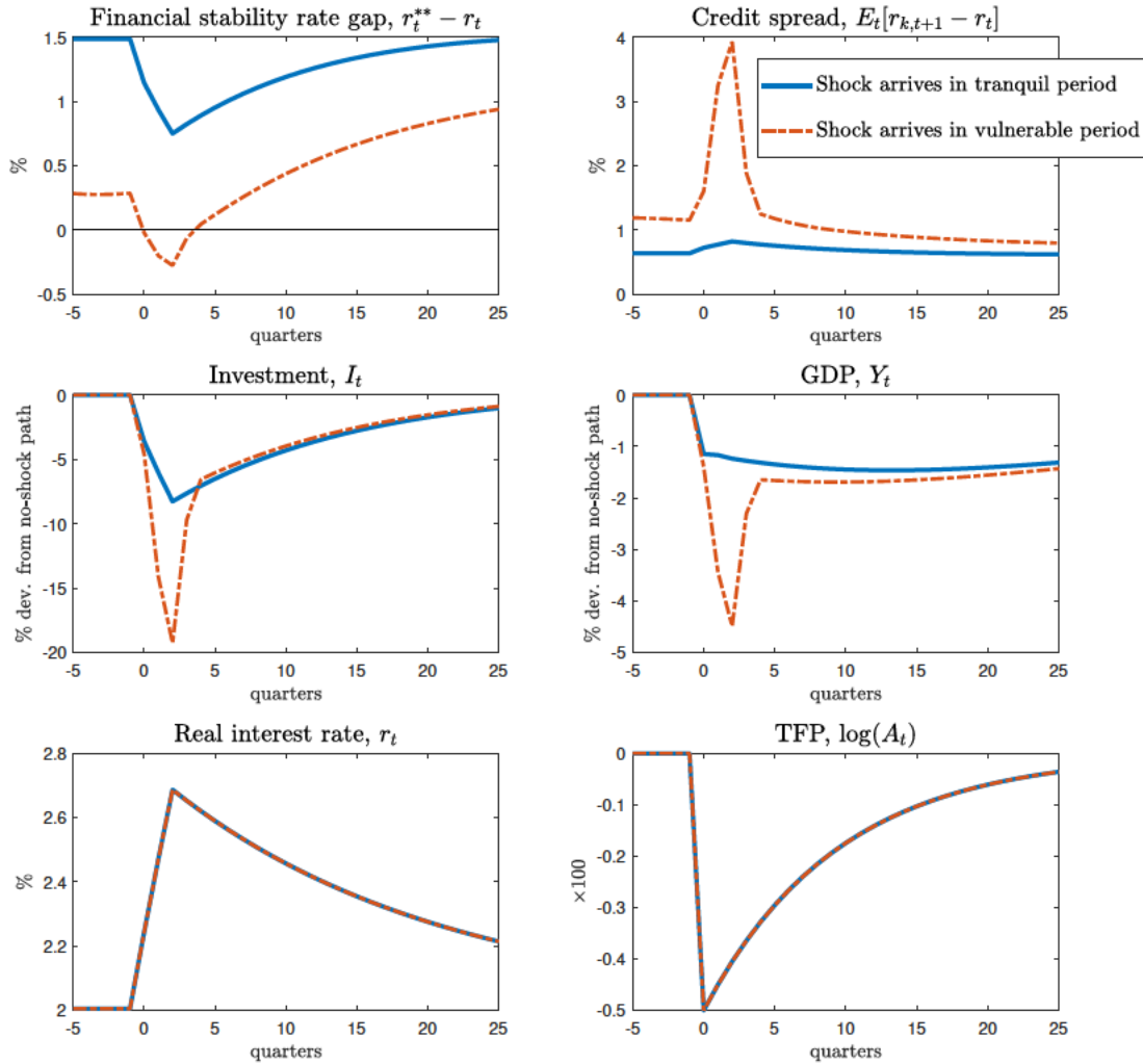
Figure 5: State Dependence
